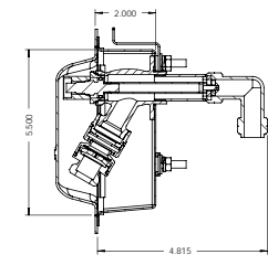
RIGHT VIEW CLOSED COUPLED VERSION, P/N AC411-02LK
